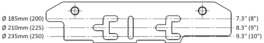
Drawing 5 Adjusting the skids
