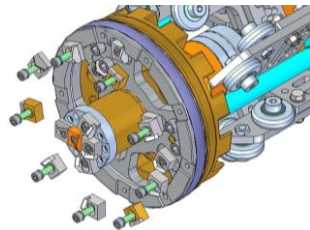
Figure 23: Diamond crown drill bit
