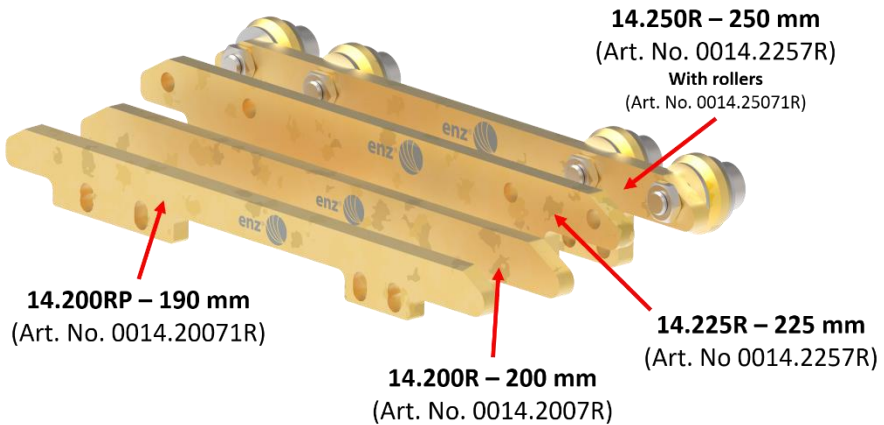
Figure 17: Skids overview
