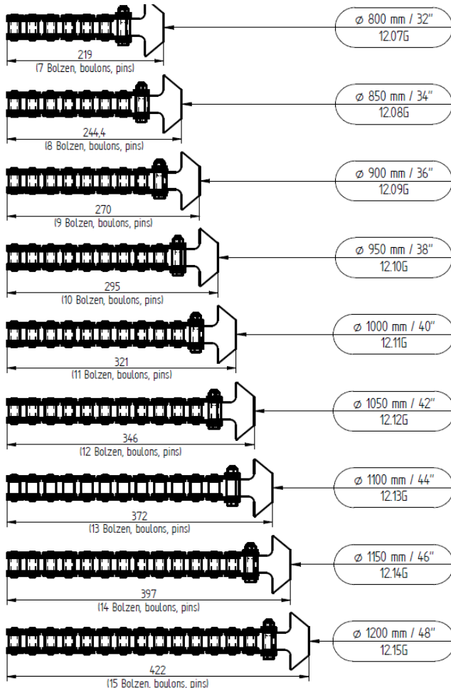
Drawing 4 All chains for 10.800R
