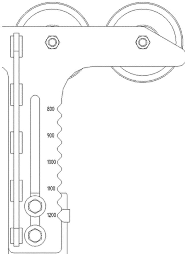
Drawing 8 Skid adjustment for 10.800R
