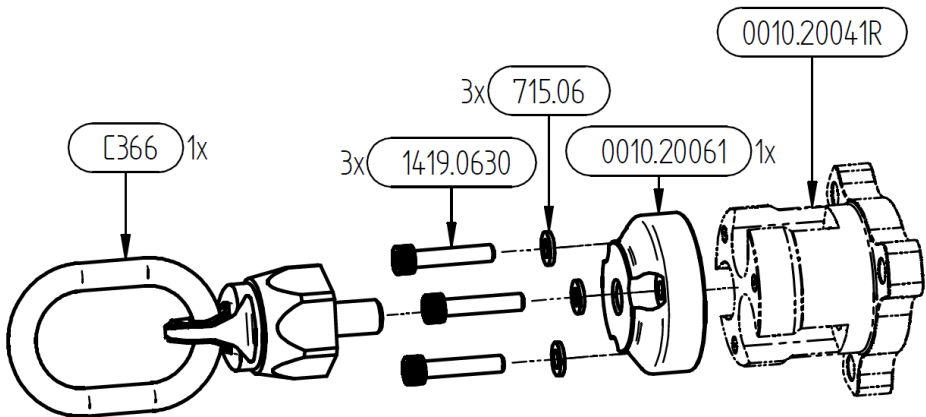
Drawing 7 Explosion of pull part 10.800R
