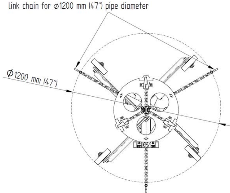
Drawing 1 Chain length greater than pipe \varnothing
