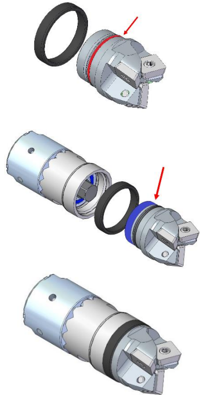
Figure 5 Conversion to milling cutter without impact
