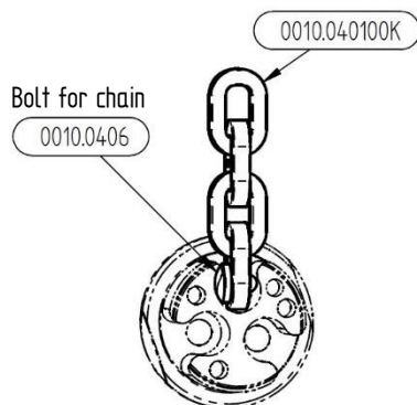
Drawing 5 All link chains for 10.060 ATR / BTR / CTR
