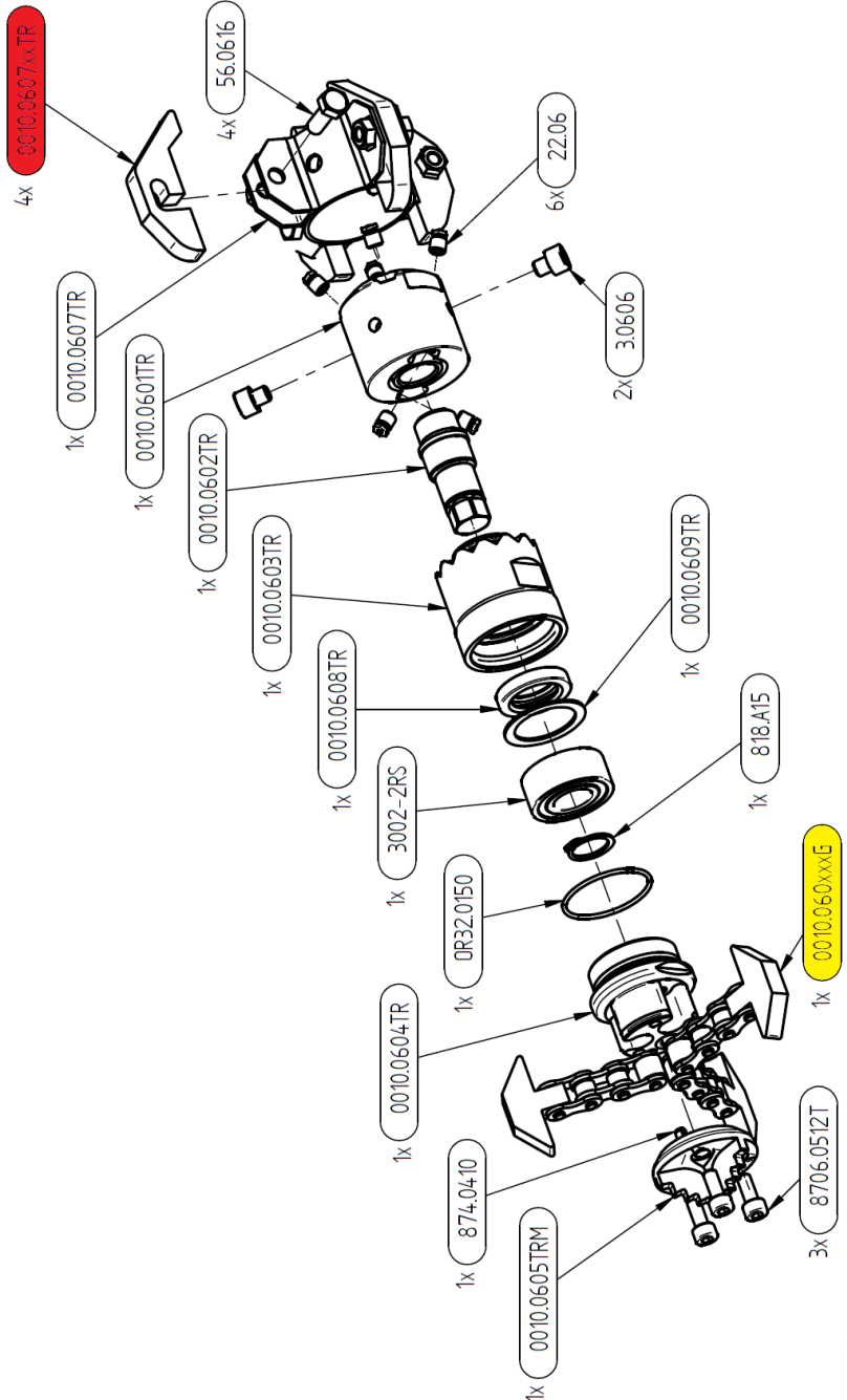
Drawing 3 Explosion 10.060BTR
