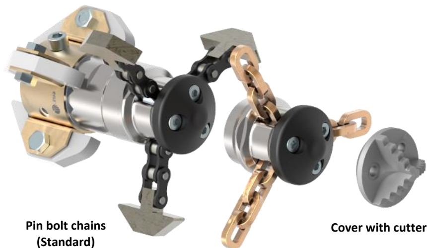
Link chains Figure 3 10.060BTR
