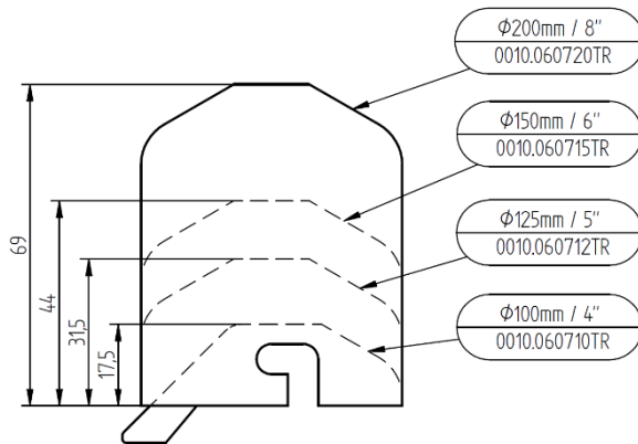
Drawing 6 All cages for 10.060 ATR / BTR / CTR
