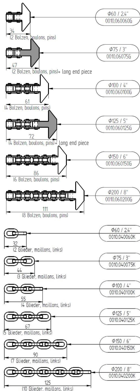
Drawing 4 All pin bolt chains for 10.060 ATR / BTR / CTR
