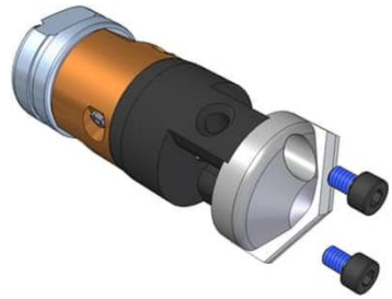
Figure 4 Converting to milling cutter
